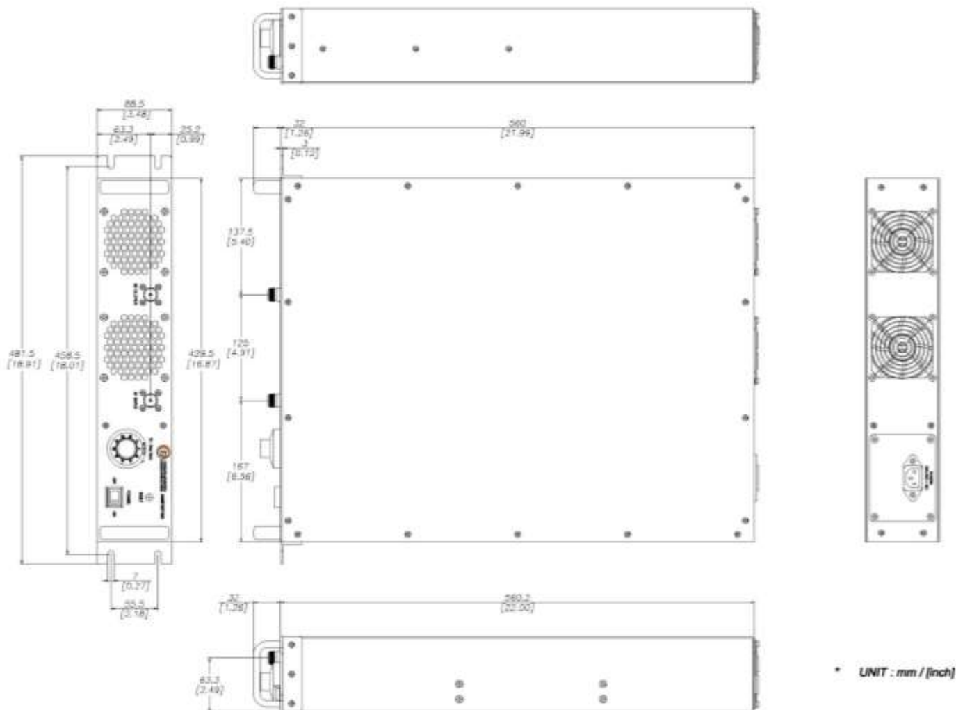
OUTLINE DRAWING-2U BASIC MODEL, NO DISPLAY WITH DMC OPTION
